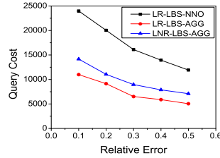
Figure 13: COUNT(schools)
