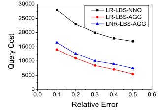
Figure 14: COUNT(restaurants)
