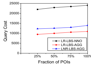
Figure 17: Varying Database Size
